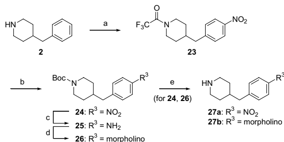
Scheme 5. Reagents: (a) TFAA, then \text{KNO}_3 , TFA; (b) aq \text{NaOH} , \text{EtOH} , then \text{Boc}_2\text{O} ; (c) \text{NH}_2\text{NH}_2 \cdot \text{H}_2\text{O} , \text{FeCl}_3 , activated C, \text{THF} ; (d) (\text{ClCH}_2\text{CH}_2)_2\text{O} , \text{KI} , \text{K}_2\text{CO}_3 , \text{DMF} ; (e) \text{HCl} , \text{EtOAc} .
